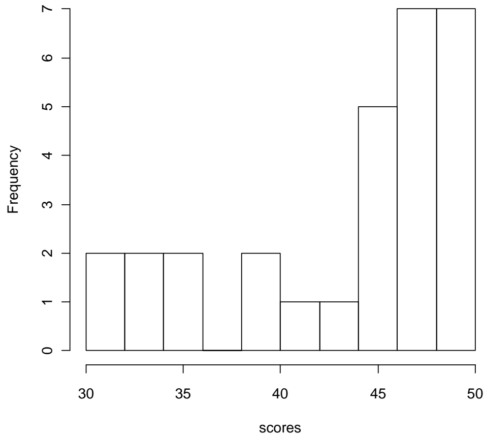
Histogram
