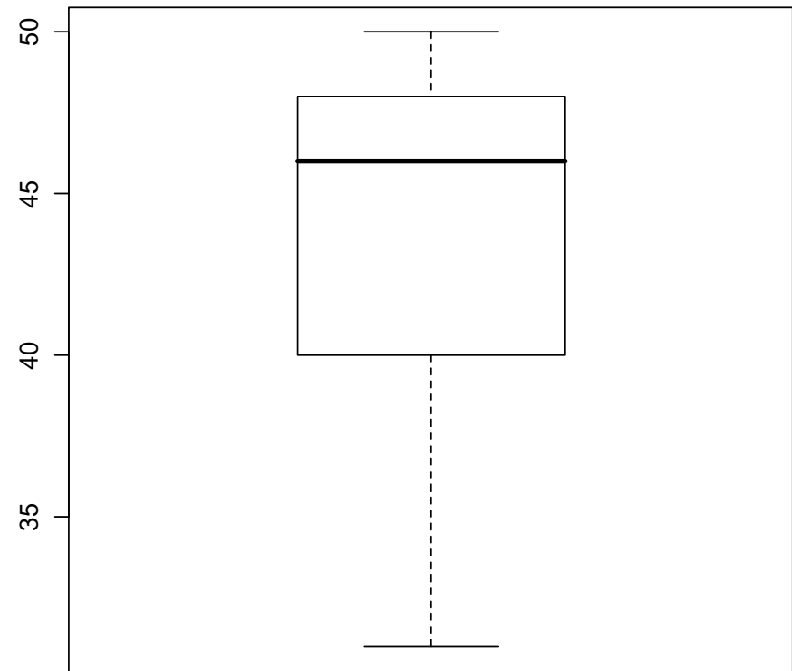
Boxplot
