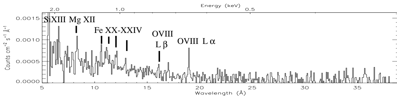
Fig. 1. The background subtracted RGS spectrum taken on 29 June 2000. The exposure was 55 ksec and includes both RGS1 and RGS2 data
