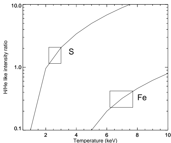
Fig. 3. The H/He like intensity ratio for sulphur and iron K\alpha as a function of temperature. We plot the observed range determined using the EPIC PN spectrum
